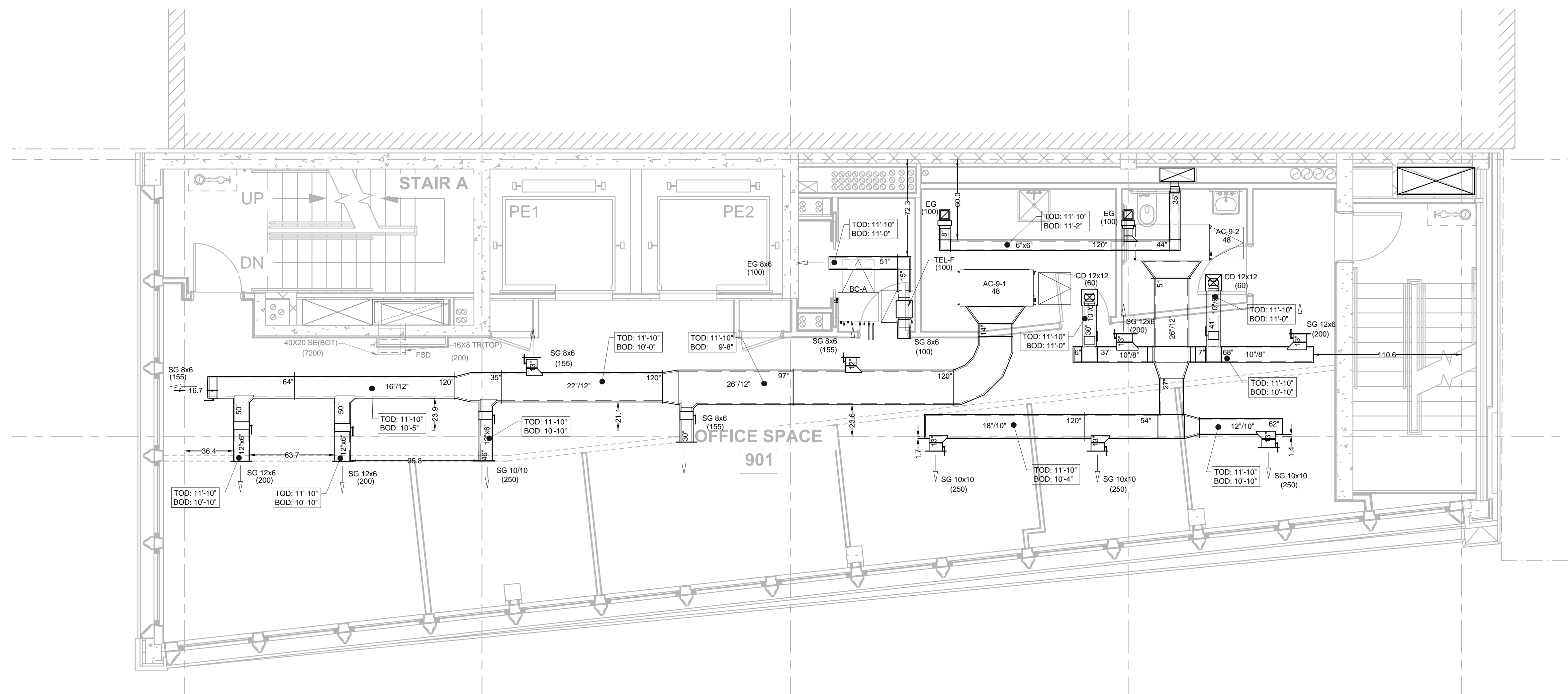
1 NINTH FLOOR HVAC SHOP DRAWING SCALE: 1/4" = 1'-0"
