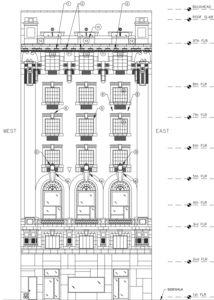
example of detailed exterior elevation drawings
