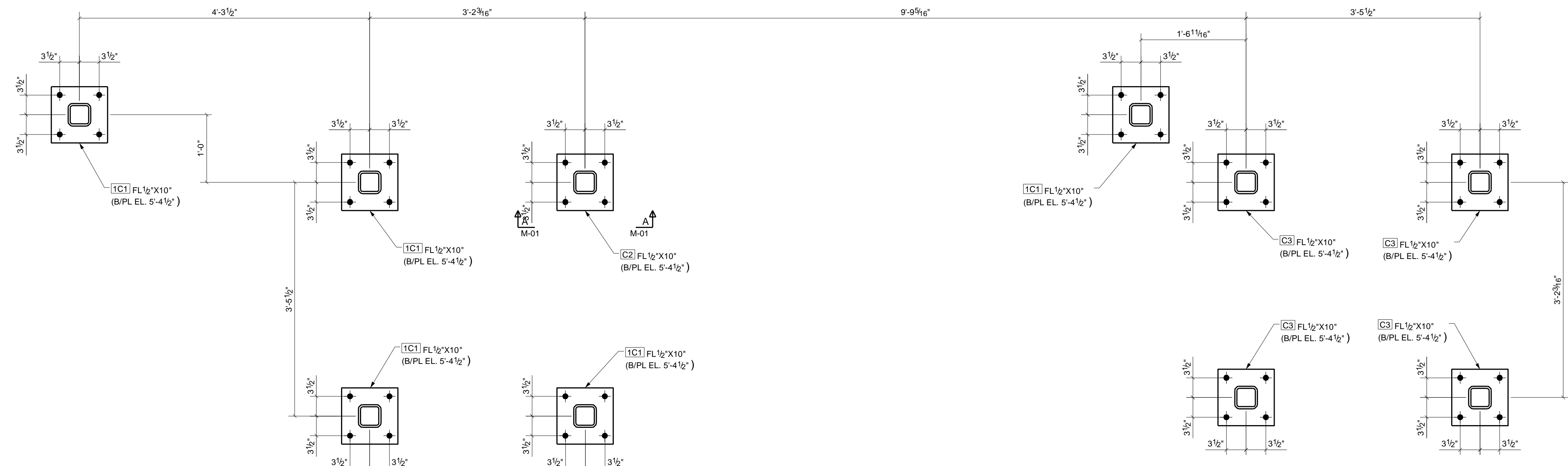
ANCHOR BOLT PLAN @ FRONT STAIR SCALE: 1" = 1'-0"
